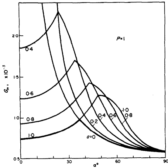
FIG. 8(b). Critical Grashof numbers of three-dimensional disturbances vs the angle of inclination: P = 1 .
